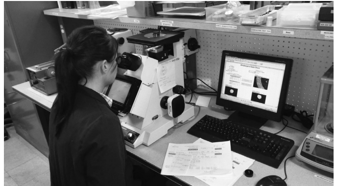
A lab service technician uses a metallurgical microscope to examine the microstructure of the metallic components in Watlow's mineral insulated metal sheathed cable, XACTPAK.
