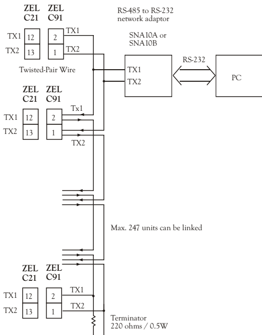
Figure 2.21 RS-485 Wiring
