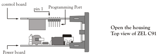
Figure 1.2 Programming Port Overview
